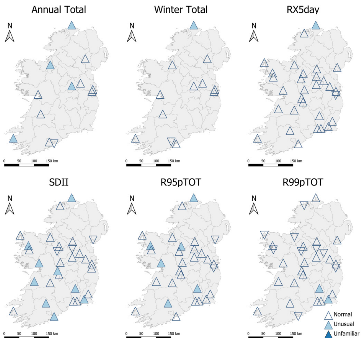
Figure 6: Signal to Noise Ratio (SNR) for precipitation indices. SNR values are categorised as 0=Normal, 1=Unusual, 2=Unfamiliar with darker triangles indicating unusual and unfamiliar. The direction of the triangle reflects the direction of the long term trend. Only indices showing the emergence of unusual climate for at least one station are plotted. See Table 2 for full description of indicators.
