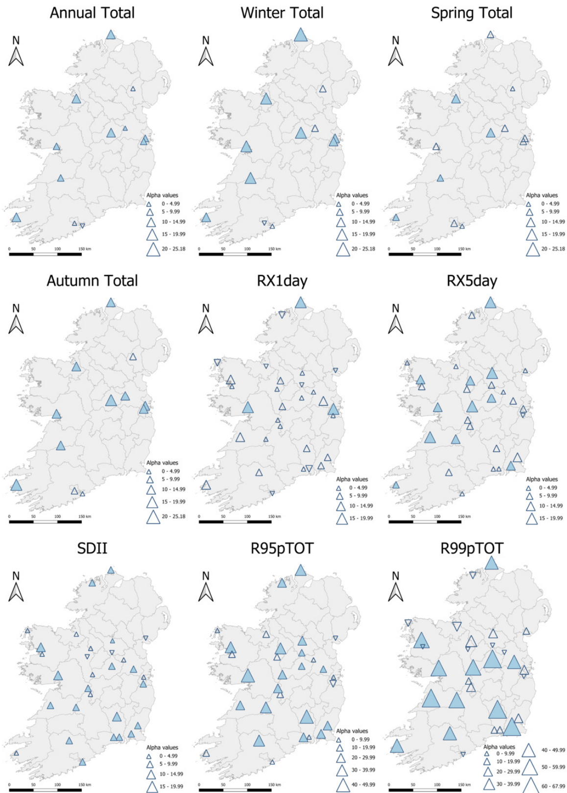
Figure 8: Alpha ( \alpha ) values as percent change per degree warming in GMST for annual and seasonal precipitation totals and annual ETCCDI precipitation extremes for each station. The size and direction of the triangle representing each station shows the magnitude and direction of change, while empty triangles indicate no significant (0.10 level) relationship with GMST. Note that summer precipitation totals are not shown as no station shows a significant relationship with GMST.
