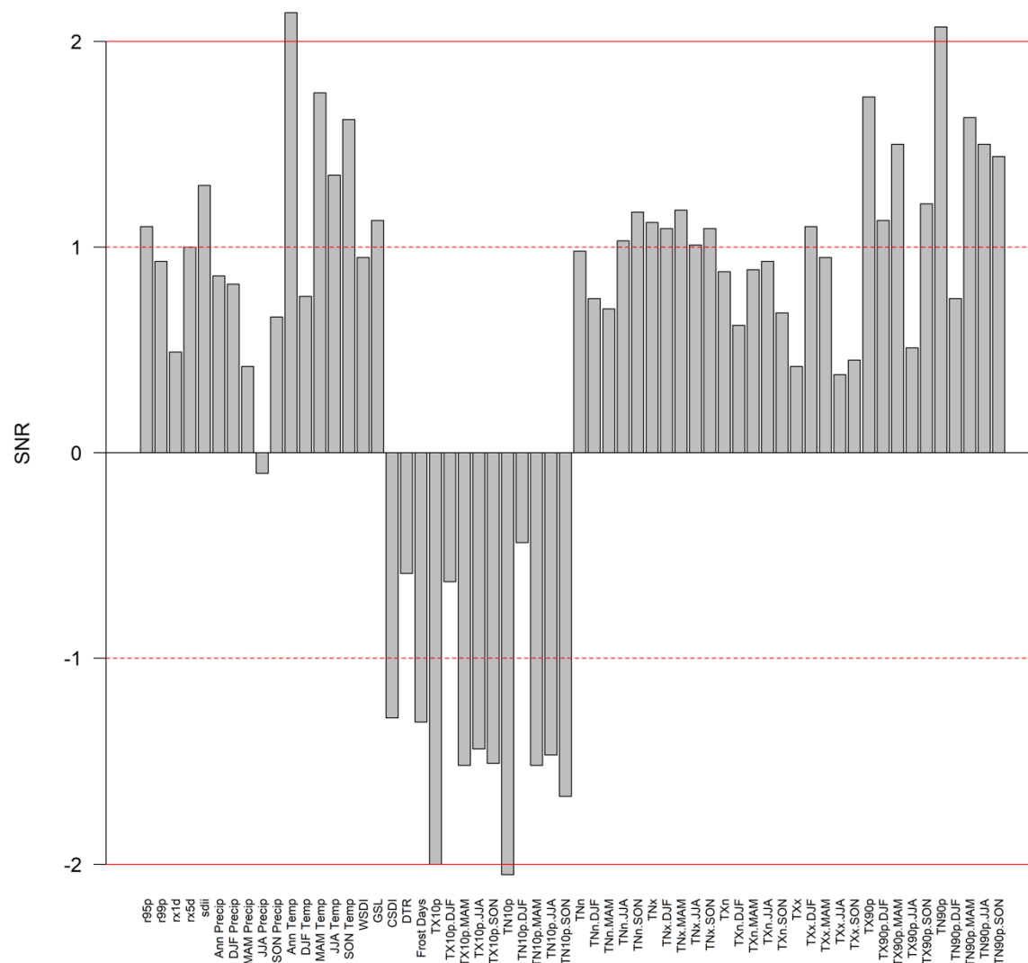
Figure 9: Barplot of the signal to noise ratio for each indicator for the Island of Ireland series. The sign of SNR shows the direction of the long-term trend. Dashed horizontal line represents the threshold for emergence of unusual climate, while the solid horizontal line represents the threshold for emergence of unfamiliar climate relative to early industrial. See tables 1 and 2 for a full description of indices.
