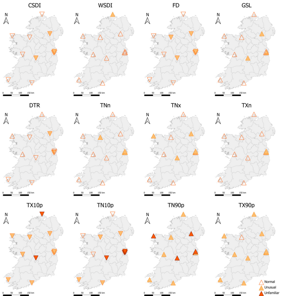
Figure 4: As Figure 2 but for annual ETCCDI temperature indices. Only indices showing the emergence of unusual climate for at least one station are plotted. See Table 1 for full description of indicators.
