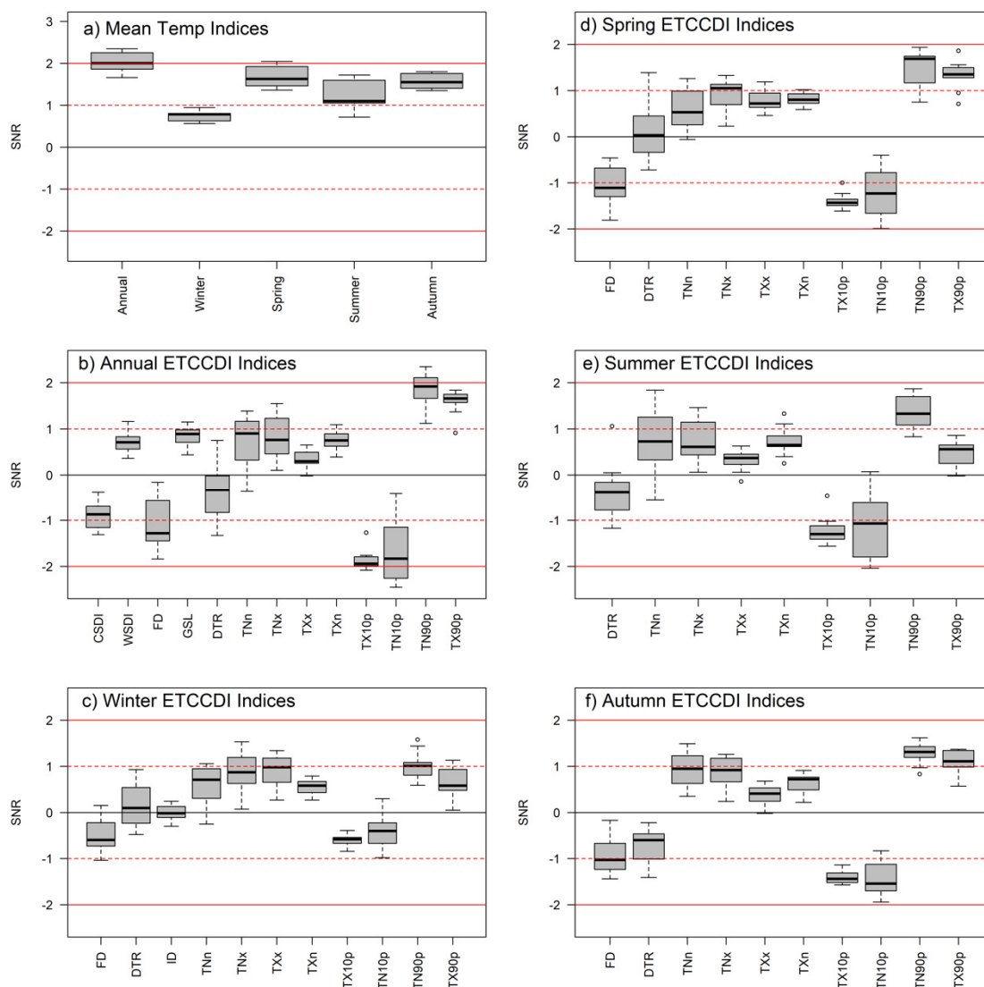
Figure 3: Boxplots of the signal to noise ratio for annual and seasonal mean and ETCCDI indices for the station sample. The dashed horizontal line represents the threshold for unusual relative to early industrial, while the solid horizontal line represents the threshold for unfamiliar climate.
