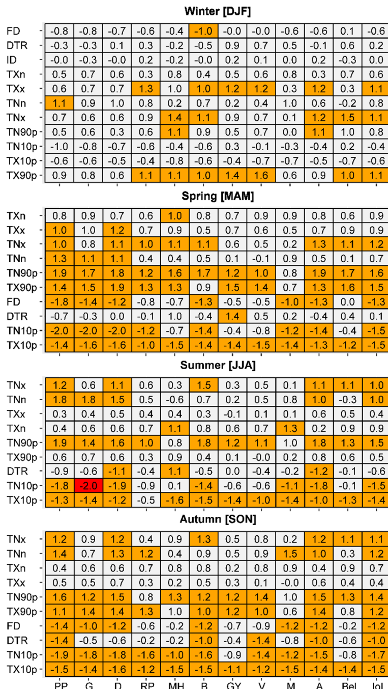
Figure 5: Heatmap showing the Signal to Noise Ratio (SNR) for seasonal ETCCDI temperature indices at each station. SNR values are categorised as Normal (no shading), Unusual (orange shading) and Unfamiliar (red shading). Stations are abbreviated as Phoenix Park (PP), Glasnevin (G), Dublin (D), Roches Point (RP), Malin Head (MH), Birr (B), Galway (GY), Valentia (V), Markree (M), Armagh (A), Belmullet (Bel), and the composite series representing the Island of Ireland (Iol). Supplementary Figures S1-S4 map the SNR for each index/season/station.
