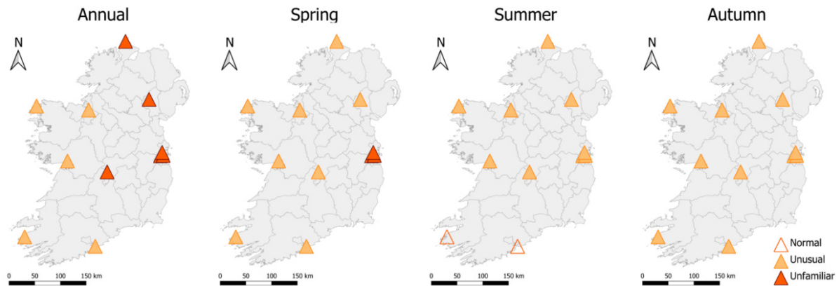
Figure 2: Signal to Noise Ratio (SNR) for annual and seasonal mean temperature for each station. SNR values are categorised as 0=Normal, 1=Unusual, 2=Unfamiliar, with darker triangles indicating unusual and unfamiliar. The direction of the triangle reflects the direction of the long term trend. Only indices showing the emergence of unusual climate for at least one station are plotted.
